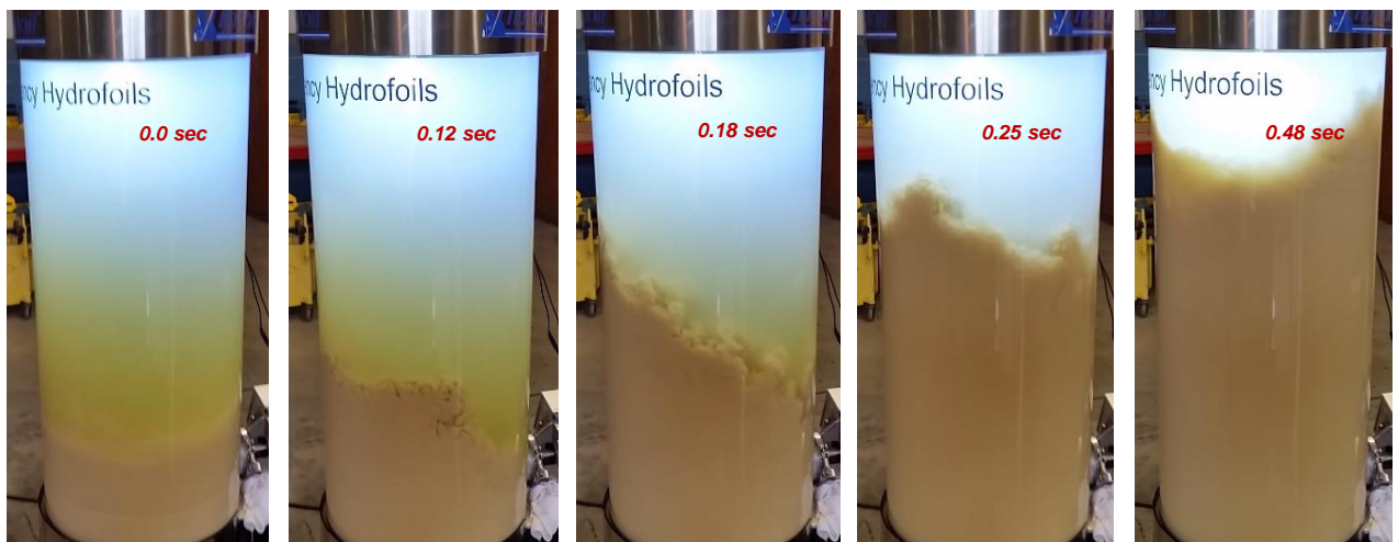
PROGRESS OF SUSPENSION OF SOLIDS Demonstration tank solution 15% solids; 210lt
